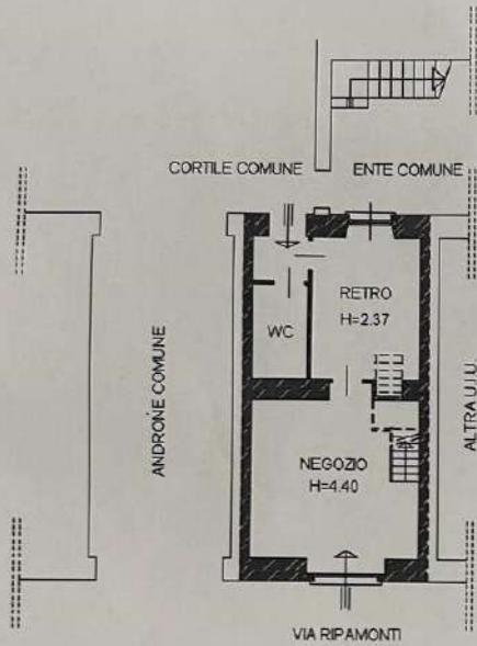
PIANO TERRA
